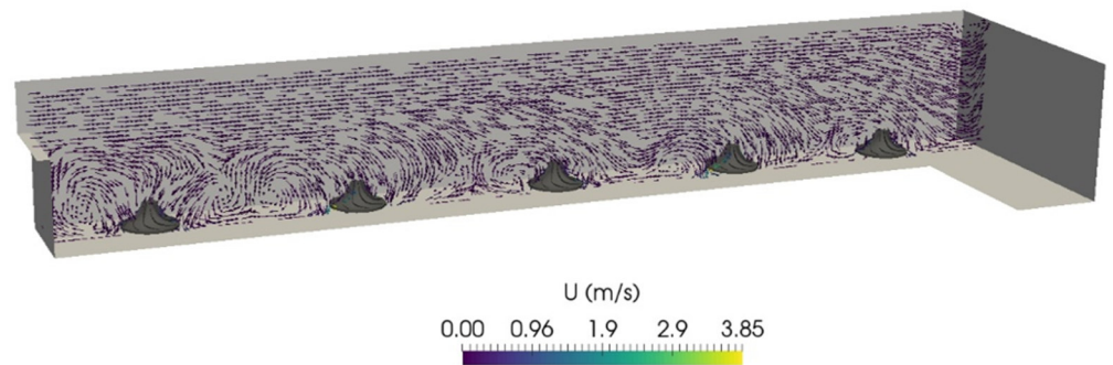
Figure 1 – CFD simulation of the anoxic section of the HRAS system, located at resource recovery facility of Breda (The Netherlands) and operated by the Waterboard Brabantse Delta.
